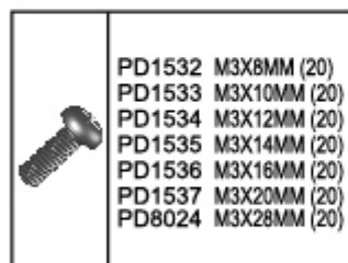
PD1532 M3X8MM (20) PD1533 M3X10MM (20) PD1534 M3X12MM (20) PD1535 M3X14MM (20) PD1536 M3X16MM (20) PD1537 M3X20MM (20) PD8024 M3X28MM (20) BT PHILLIP MACHINE SCREW 圓頭十字螺絲
