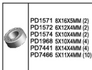
PD1571 8X16X5MM (2) PD1572 6X12X4MM (2) PD1574 5X10X4MM (2) PD1968 5X10X4MM (4) PD7441 8X14X4MM (4) PD7466 5X11X4MM (10) BALL BEARING 滾珠軸承
