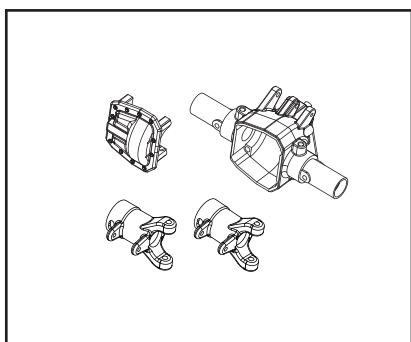
PD90600S1 Scale Axle Set (F) 像真齒輪箱組 (前)
