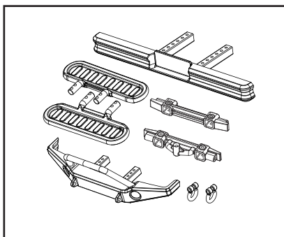
PD90606S1 Side Guard & F/R Bumper Set 側板+前後防撞板
