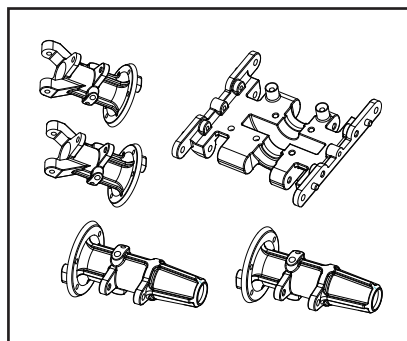
PD90447S1 Center Diff Mount 中差固定座
