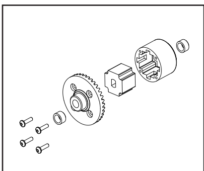
PD90442S1 Differential Set 差速組
