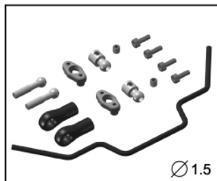
PD9200-2 REAR SWAY BAR SET(BLACK) 防傾桿組(黑)
