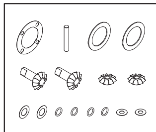
PD7746 DIFFERENTIAL GEAR SET 差速齒輪組
