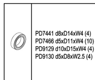
BEARING 滾珠軸承
