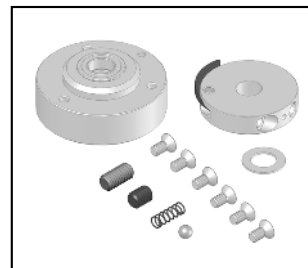
PD2271 2 SPD CLTCH HUB HARDWARE
