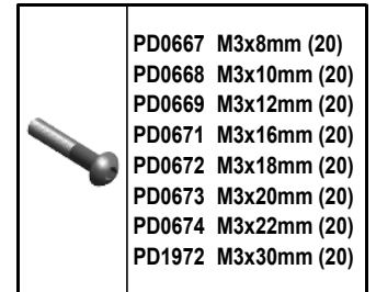
BT MACHINE SCREW
