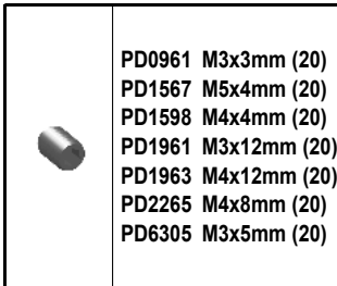
SET SCREW
