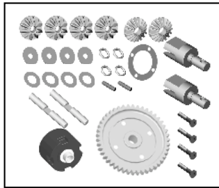
PD1800 DIFFERENTIAL SET CENTER,S3
