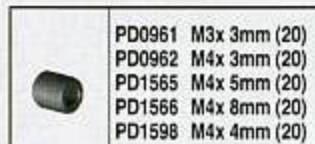
SET SCREW
