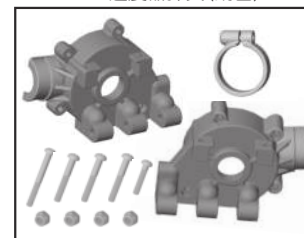
PD1483 DIFF CASE/BULKHEAD, 差速箱本體
